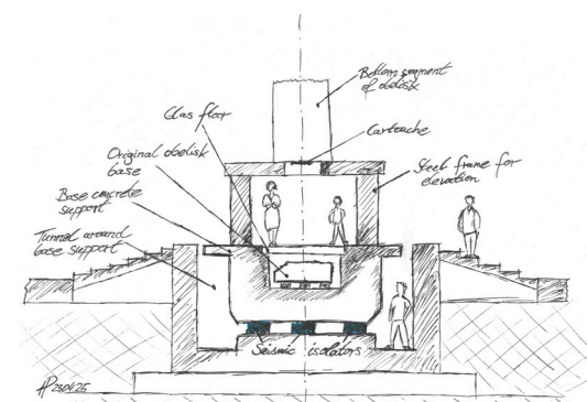
Schematic diagram and cross-section of the system.
